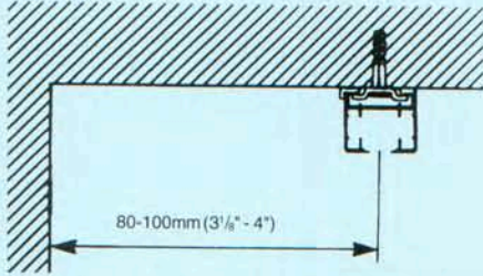
Swing clamp #3825 spaced approx. 60cm (24") o.c.
