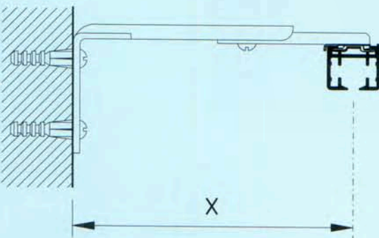
Wall mount with bracket #3832 and extension bracket #0829 or #0831
