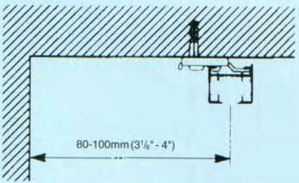
Bracket #3832 spaced approx. 60cm (24") o.c.
