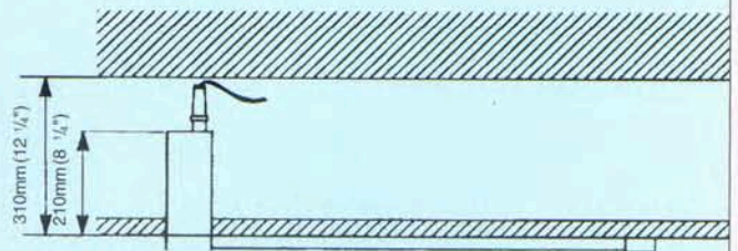
System ceiling mounted with motor recessed above
