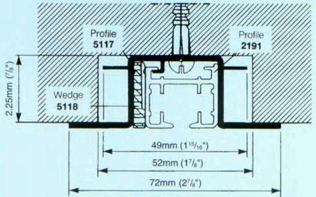
Profile recessed into ceiling with motor below rail or rail and motor recessed into ceiling
