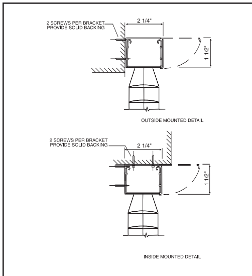
Custom 2" NuWood™ mounting detail.
