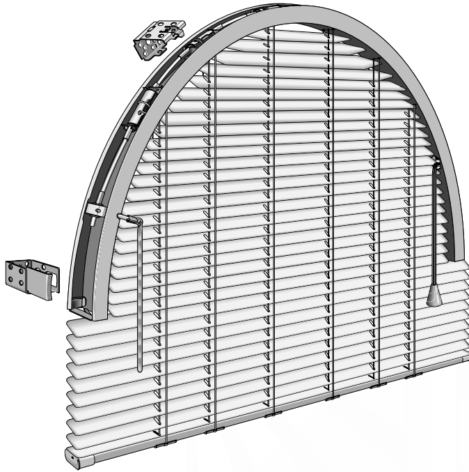
Headrail
