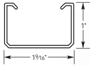
Headrail
