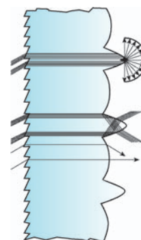
Front Side Vertical lenticular lenses for horizontal light distribution.
